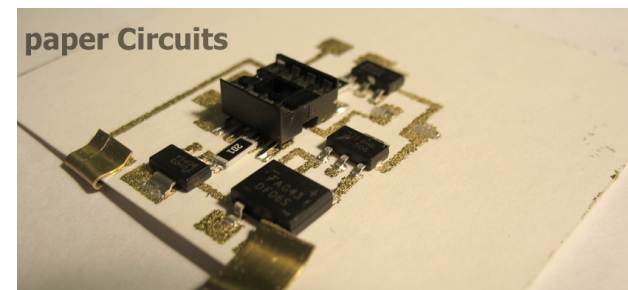
Figure 4. Gold leaf circuit for controlling a SMA wire and rectifying external AC power.
